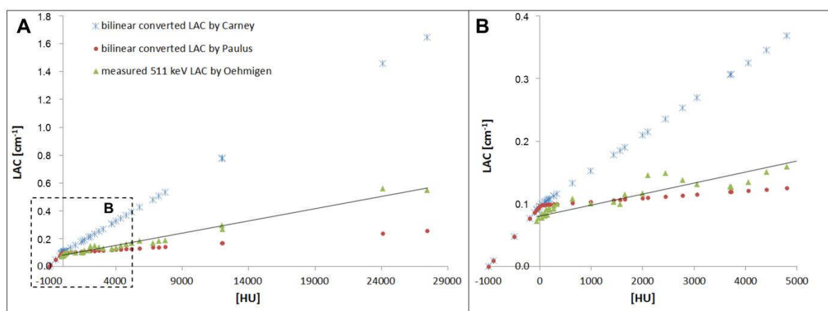
Figure 6: The line of best fit for the measured HU and LAC values (Oehmigen et al.) of the materials (green triangles) is located between the two calculated LAC values of Carney et al. (blue x's) and Paulus et al. (red circles). Note that the blue and red data points were not measured by Carney, nor by Paulus and colleagues. Instead, all data points were derived from the CT HU values of all material samples evaluated in this study by
